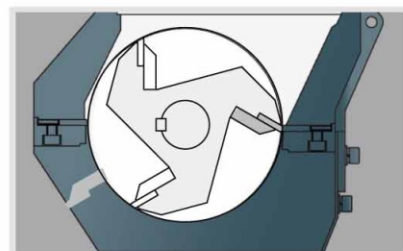
SG-16N/16D/SG-20NC Structural Drawing of Staggered Blades
